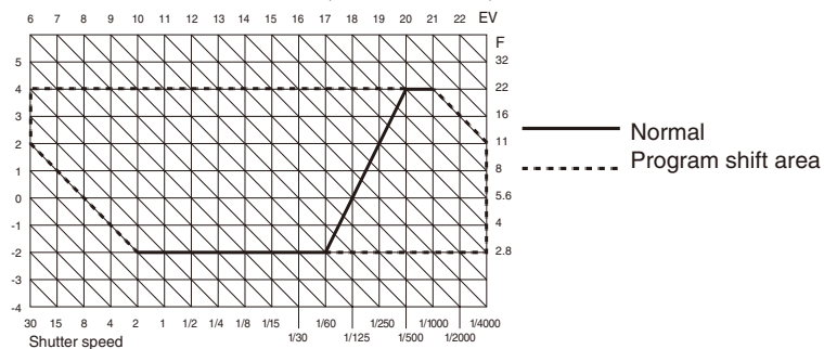
645DF program shift chart
